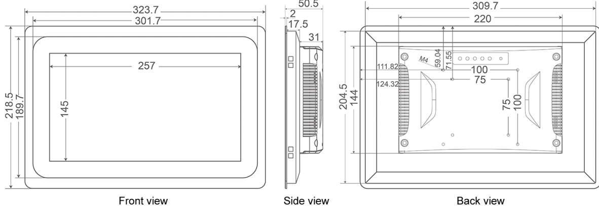
11.6" Touch Monitor
