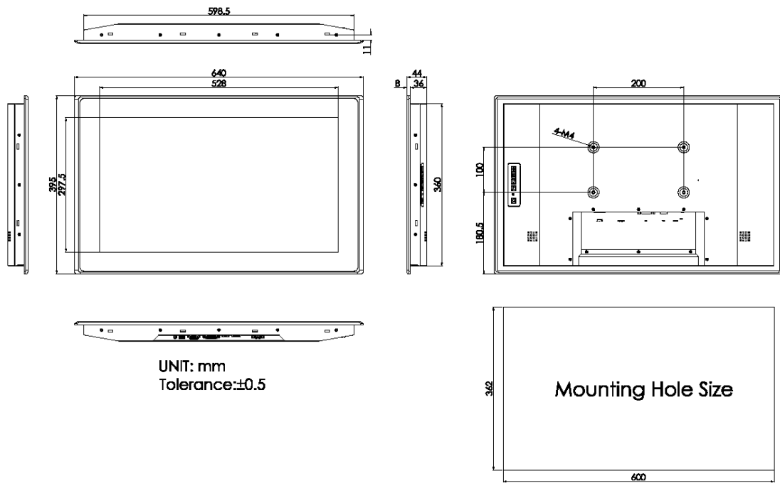
Figure 1.11: Dimensions of ARCDIS-124APG(H)
