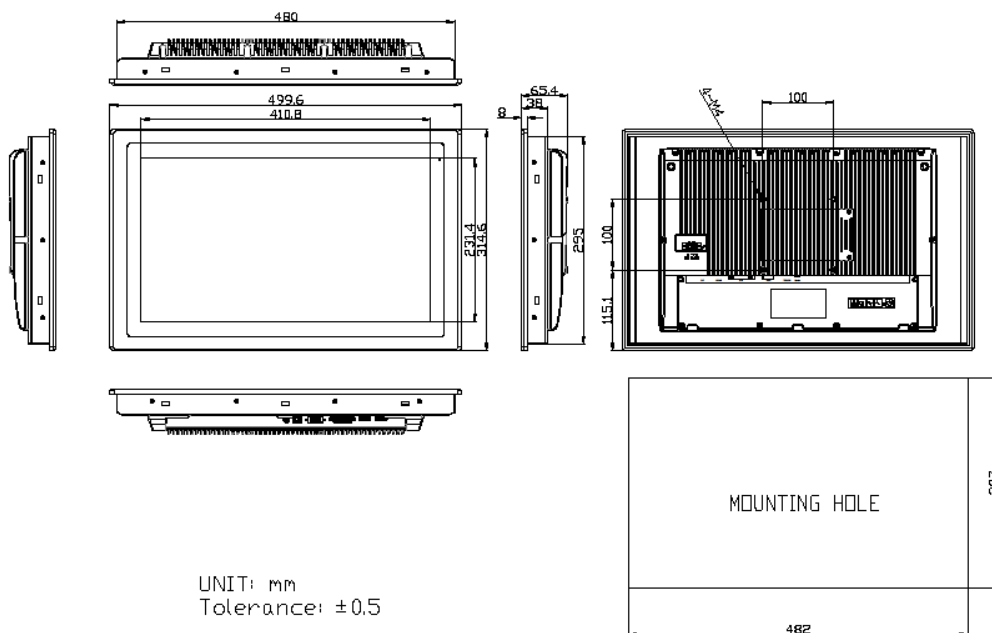
Figure 1.7: Dimensions of ARCDIS-117APRG(H)
