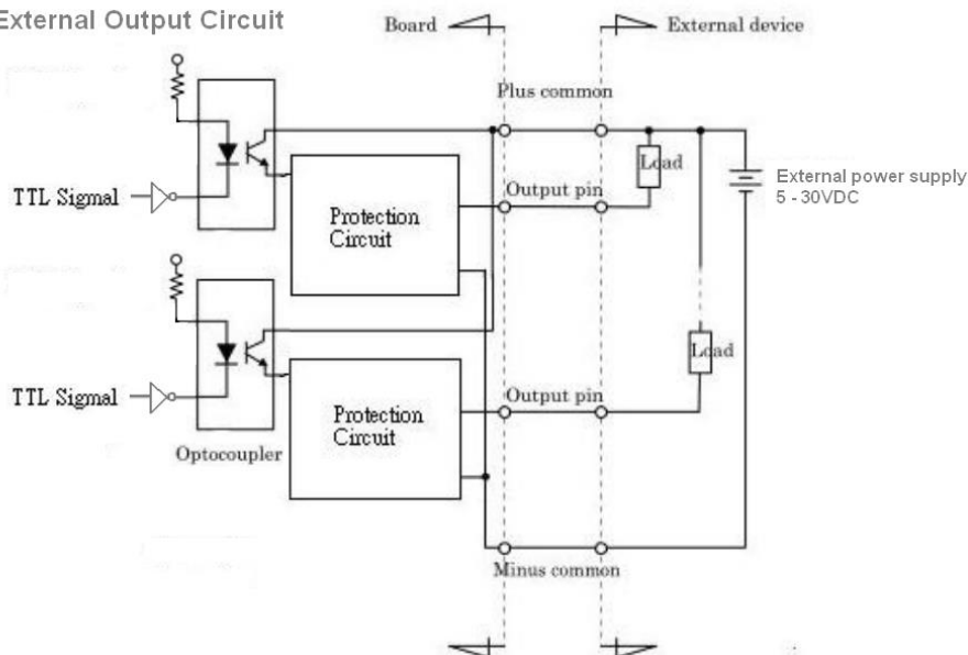
External Output Circuit
