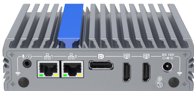
WIFI AUDIO LANx2 DP HDMIx2 DC12V WIFI
