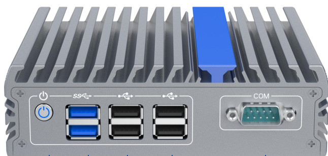
POWER USB3.0x2 USB2.0x4 COM
